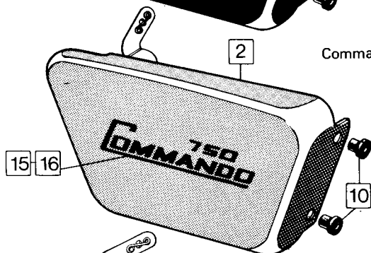
Commando 750 Roadster
